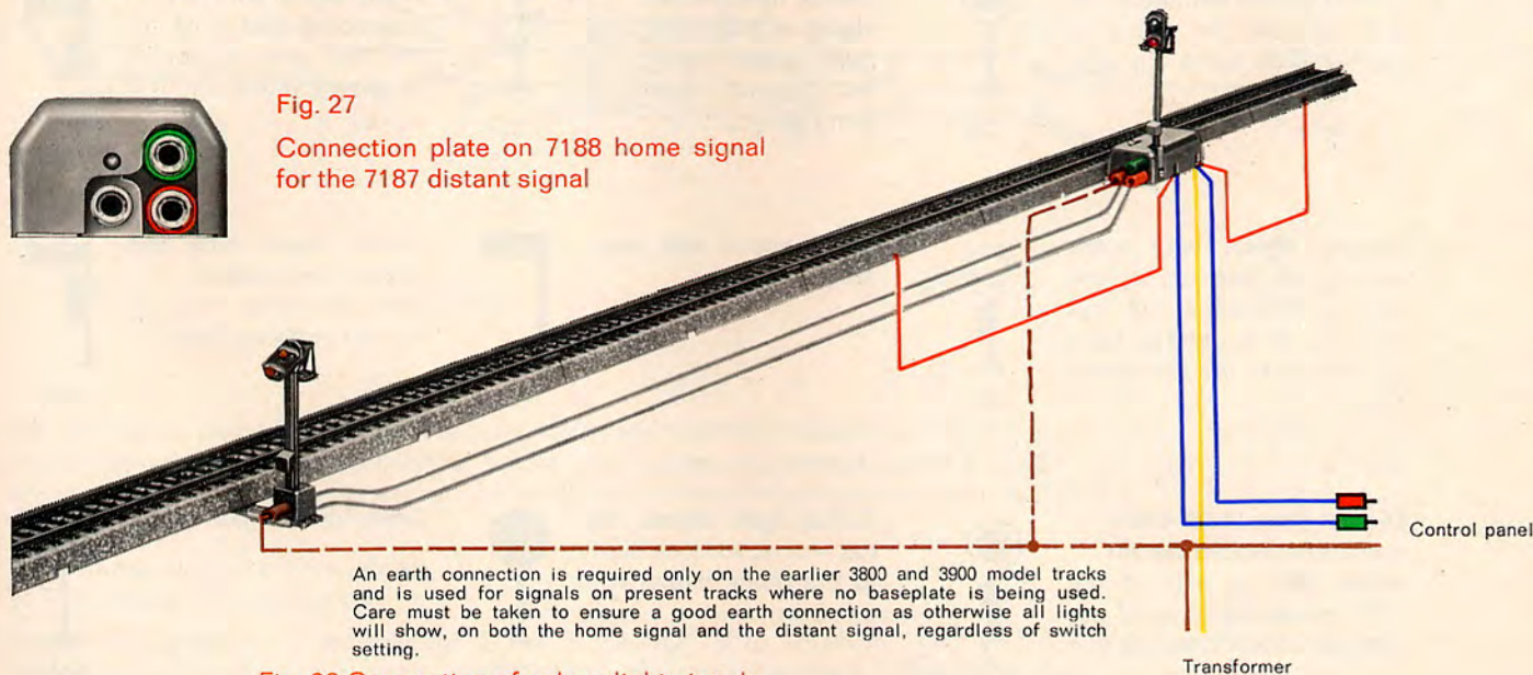
Fig. 26 Connection of colour-light signals
