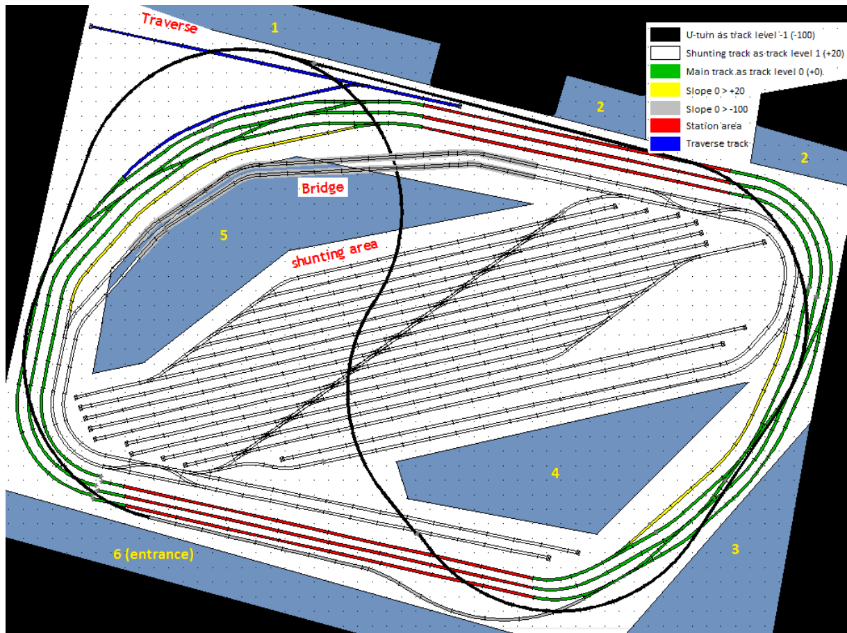
Sketch 4: Track layout with table and floor surfaces.
