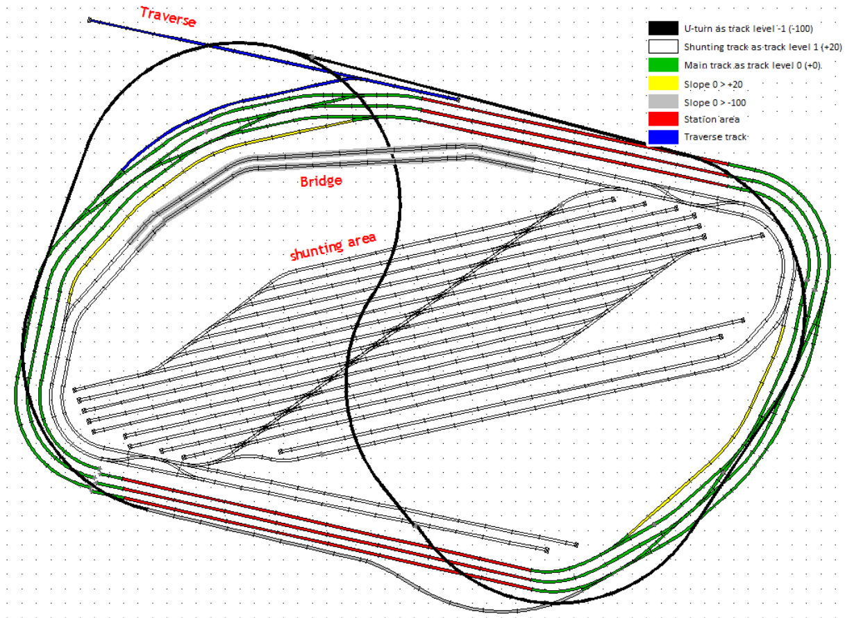
Sketch 1: Track layout
