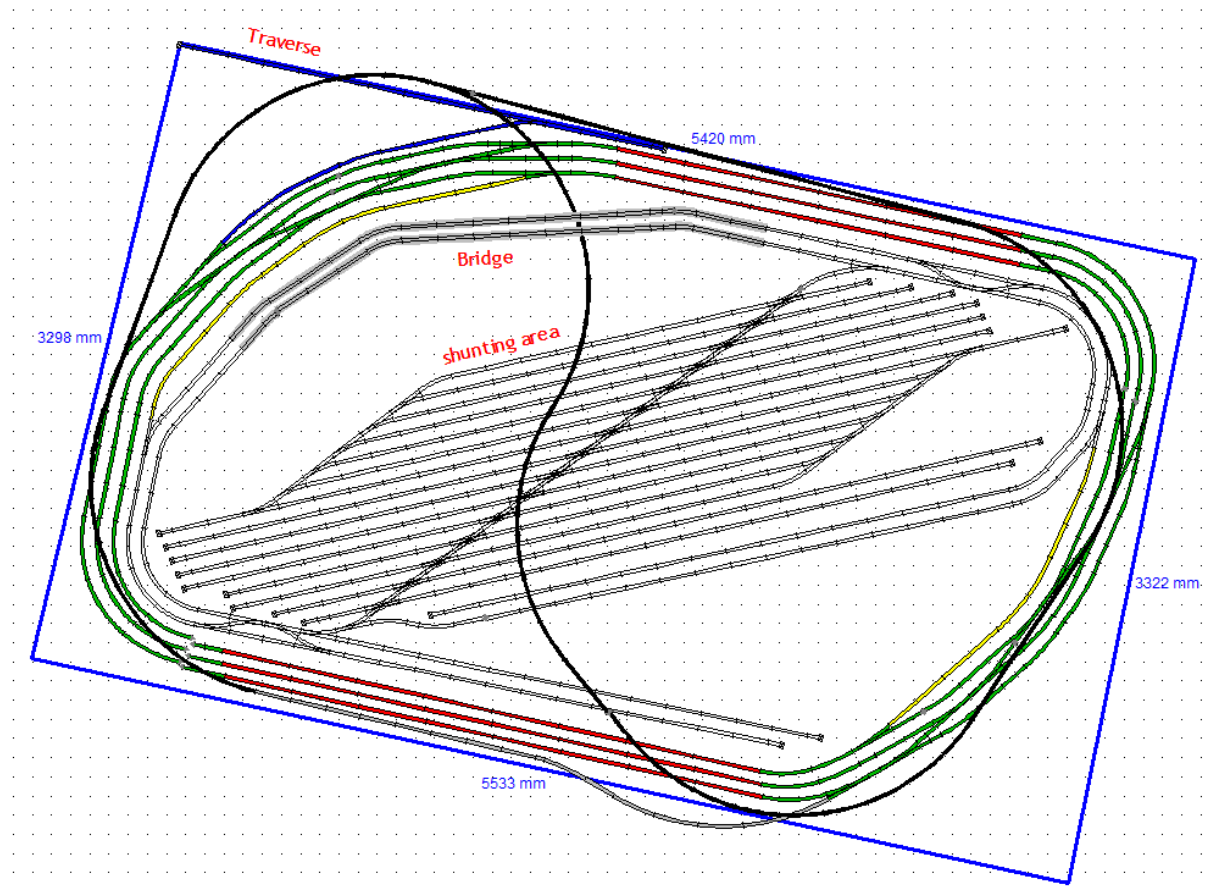
Sketch 3: Track layout with prox. table dimensions.
