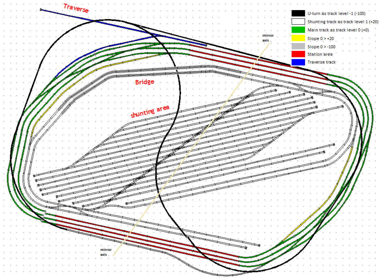
Sketch 2: Track layout with mirror line.
